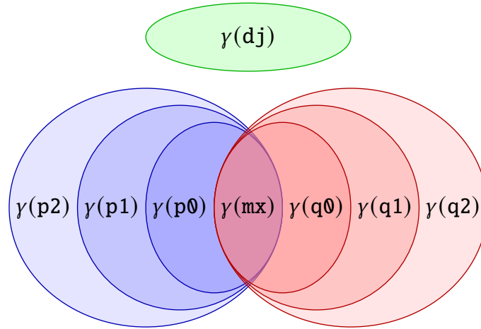
Figure 5.2: Venn diagram representation of the set inclusion relation between the concretizations of each regular type. Such relation then induces the order relation of the eterns abstract domain.
